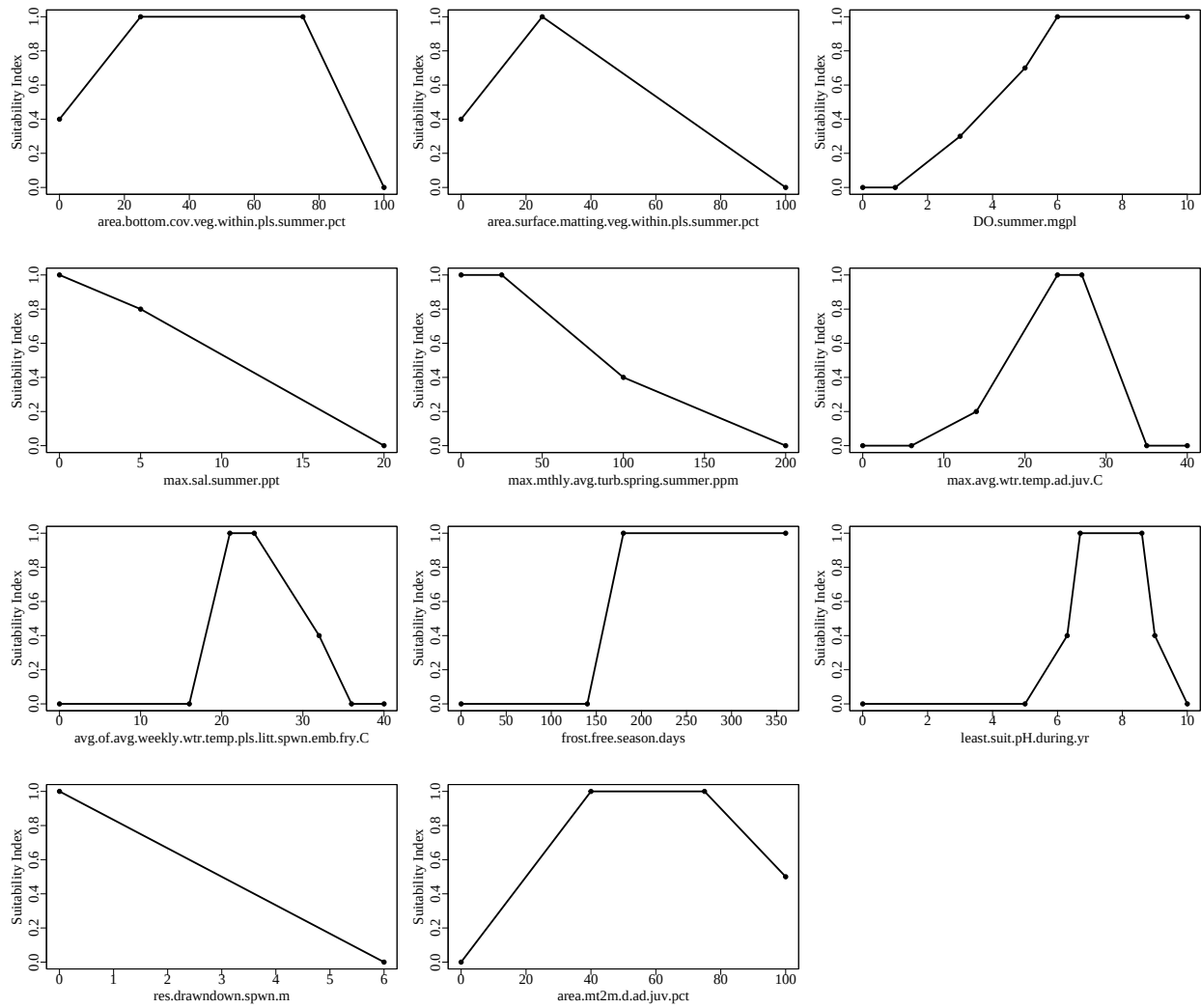
Figure 1. Suitability index graphs for variables included in the redearsunfishLac model in ecorest.
